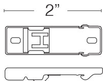
Single ceiling-mounted bracket
