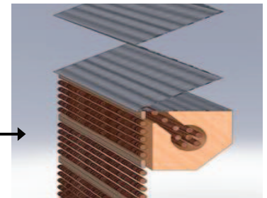
TriLight intermediate connecting rail detail view
